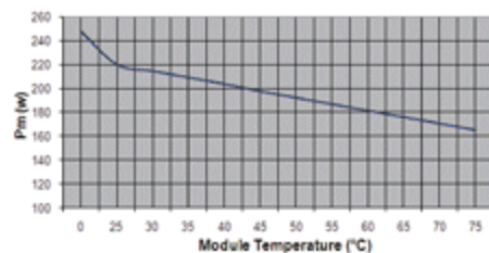
Power Output of Conventional modules over temperature
