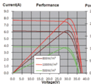
Electrical performance (Cell temperature: 25°C)
